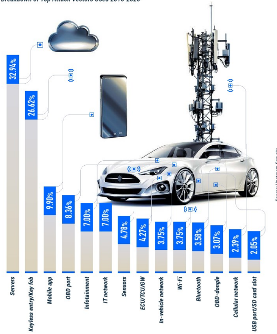
Breakdown of Top Attack Vectors Used 2010-2020
